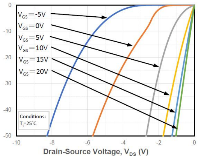
Figure 8. Reverse Output Characteristics at T_j = 25^\circ C
