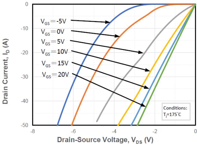
Figure 9. Reverse Output Characteristics at Tj = 175°C
