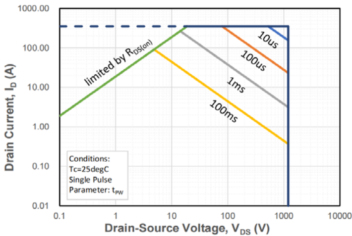
Figure 15. Safe Operating Area
