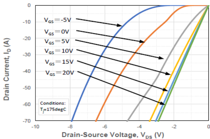
Figure 9. Reverse Output Characteristics at Tj = 175°C
