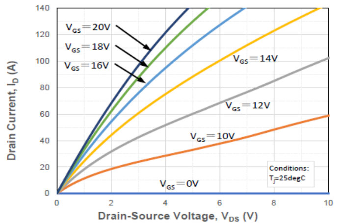
Figure 2. Output Characteristics T j = 175°C
